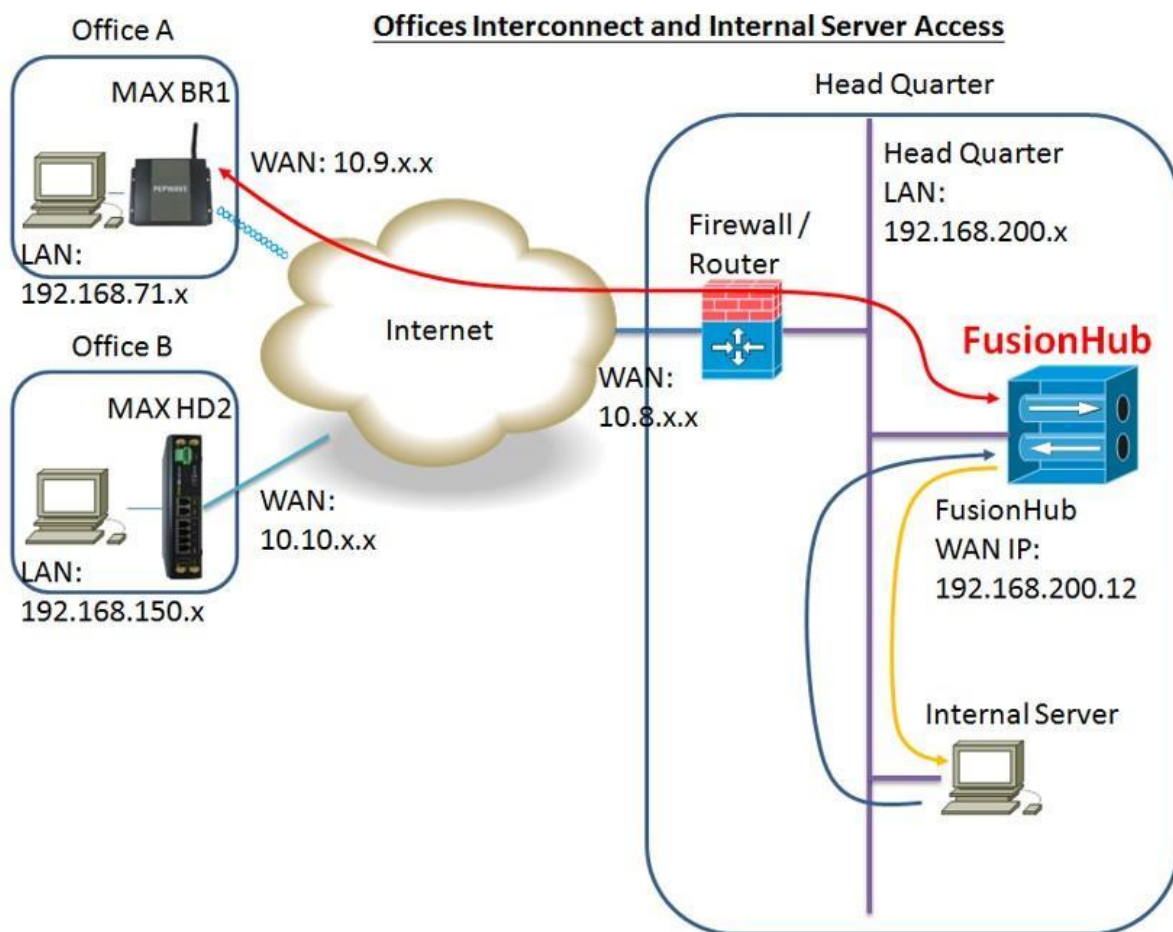
Figure 5.2 Offices interconnect
